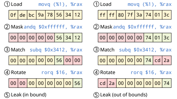
Fig. 7: Using mask, subtract, and rotate we can selectively filter data in speculative execution to match prior observations, eliminating a large amount of noise.
